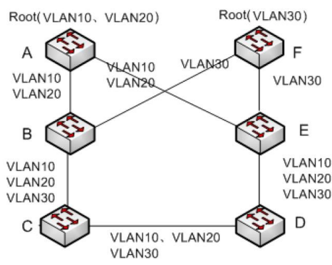
Рис. 190. STRP -VLAN-Based
